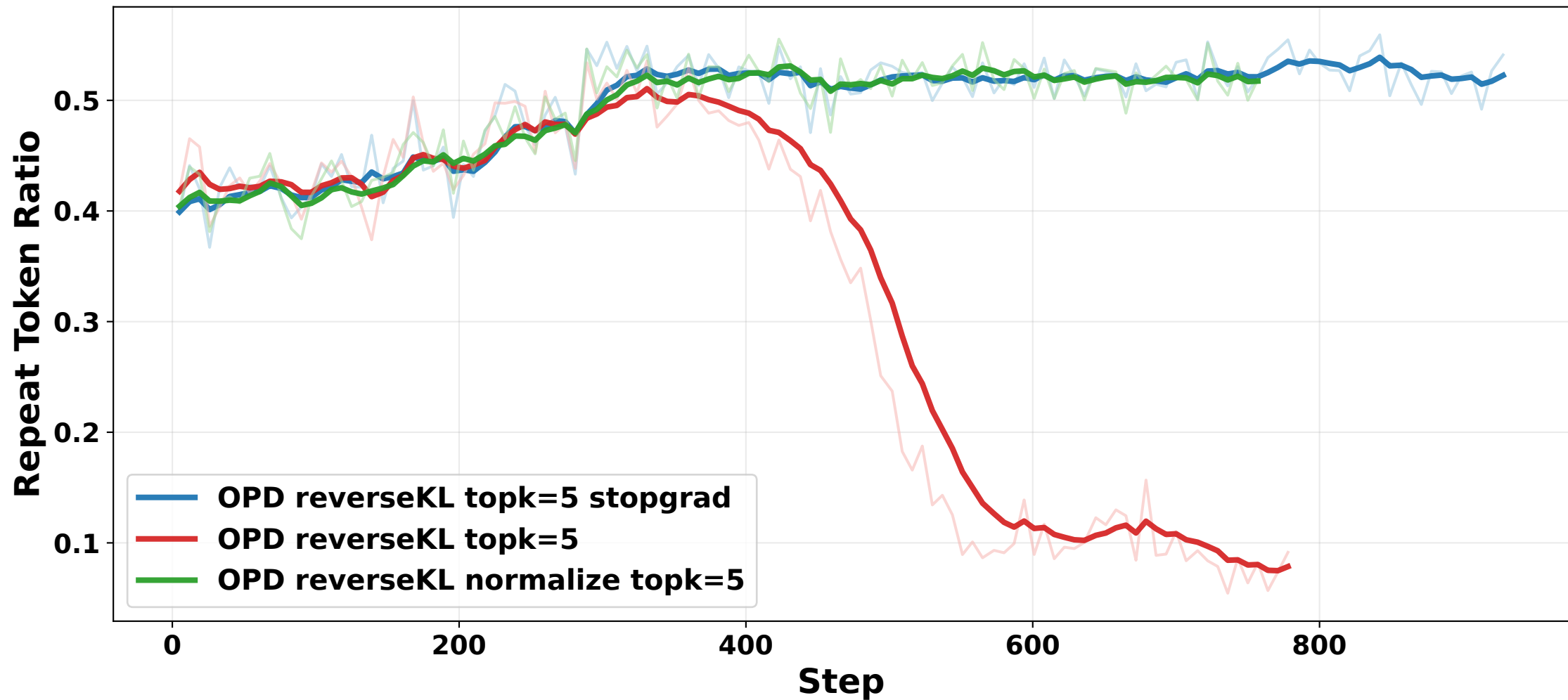
train/repeat_ratio
